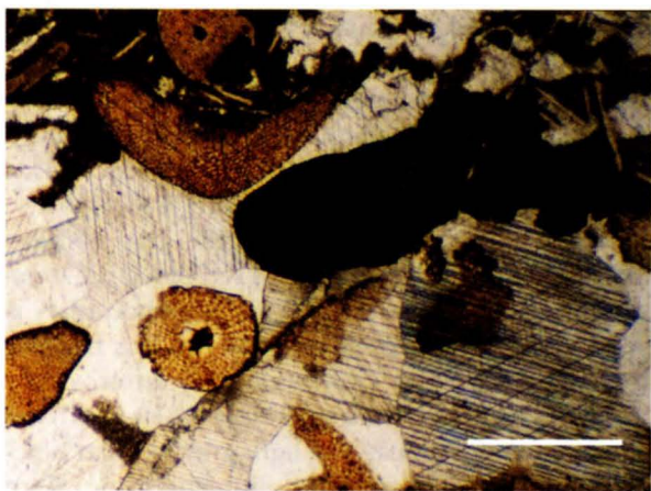
Fig. 3.22 Lower Member of the Prehodavci Formation: grainstone with echinoderm fragments and a completely Fe-Mn incrustated intraclast (section TV1). Scale bar is 1 mm long.
