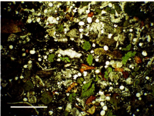
Fig. 3.52 Member 1 of the Travnik Formation: calcarenite with abundant glauconite grains, radiolarians, phosphate grains and filaments (section MA1). Scale bar is 1 mm long.
