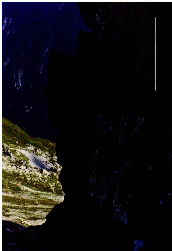
Fig. 3.42 Upper part of the Sedlo Formation: greenish rudstone – packstone and red siliceous limestone (Travnik structural unit of the Mt. Mangart saddle, section MA1). Section is in overturned position. Scale bar is 1 m long. Photo Rafael Marn.
