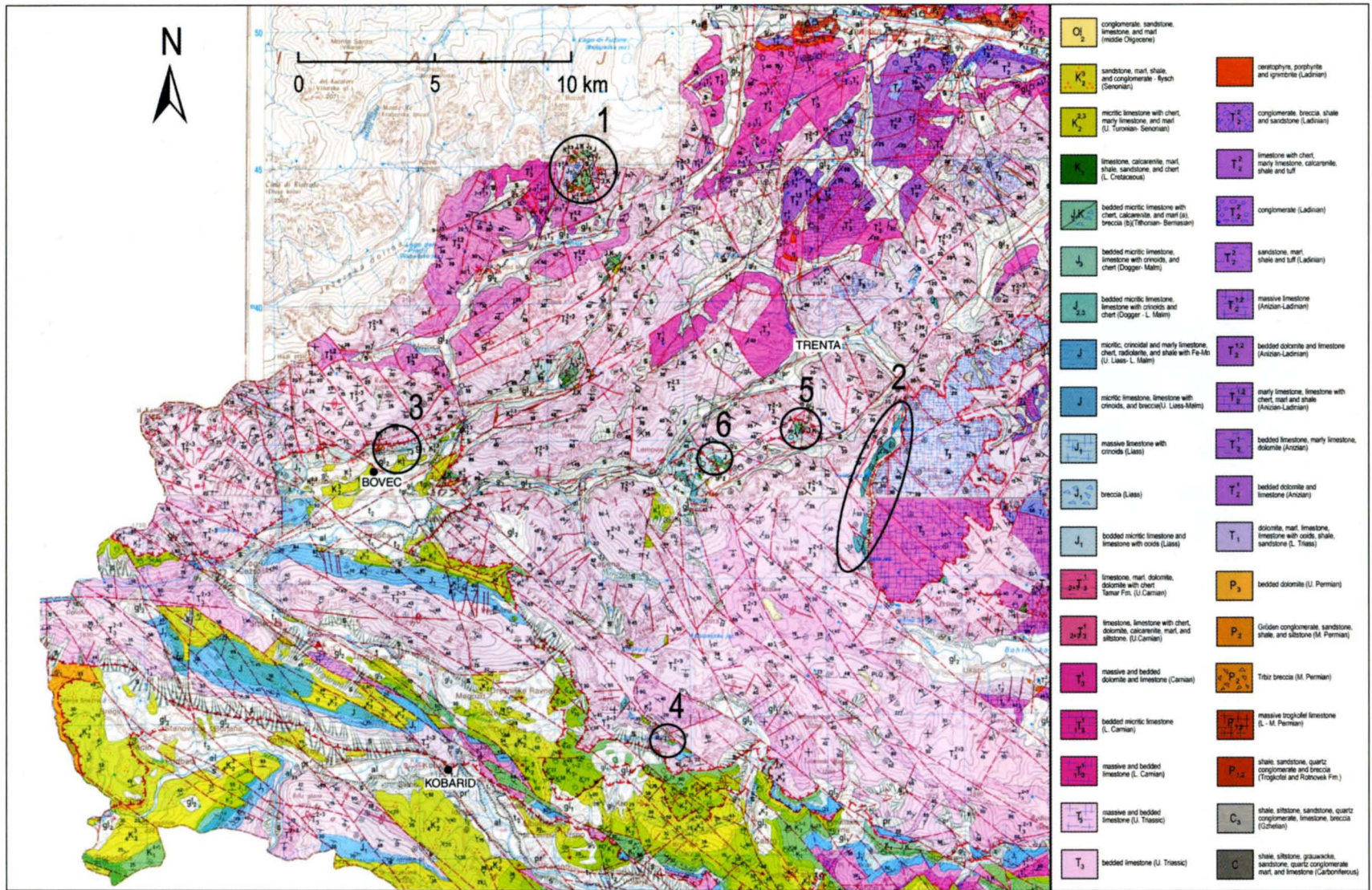
Fig. 1.5 Basic geological map of Yugoslavia, sheets Tolmin and Videm (Buser 1986) and Beljak and Ponteča (Jurkovšek 1986) with investigated localities marked: 1. Mt. Mangart Saddle, 2. Triglav Lakes Valley, 3. Ravni Laz, 4. Lužnica Lake, 5. Čisti Vrh, 6. Vas na Skali.
