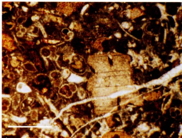
Fig. 3.21 Lower Member of the Prehodavci Formation: bioclastic limestone with echinoderm fragments and planktic foraminifers (section R1). Scale bar is 1 mm long.
