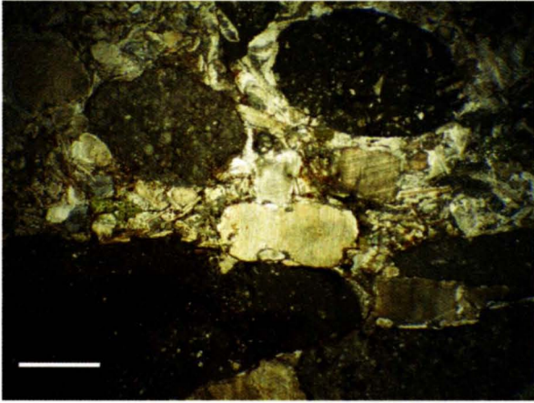
Fig. 3.51 Member 1 of the Travnik Formation: breccia with echinoderm fragments, glauconite and abundant lithoclasts of the bioclastic limestone of the Sedlo Formation, mudstone lithoclasts and lithoclasts of siliceous limestones of the Skrile Formation (section MA1). Scale bar is 1 mm long.
