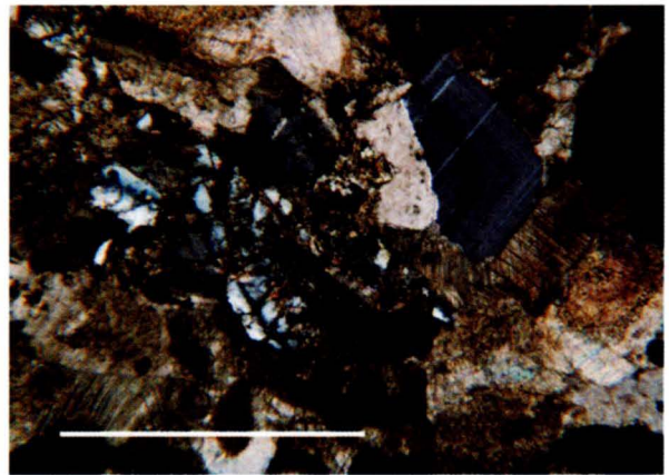
Fig. 3.66 Member 4 of the Travnik Formation: breccia with echinoderms and euhedral detritic grain of bytownite-anorthite feldspar (section MA1). Scale bar is 1 mm long.
