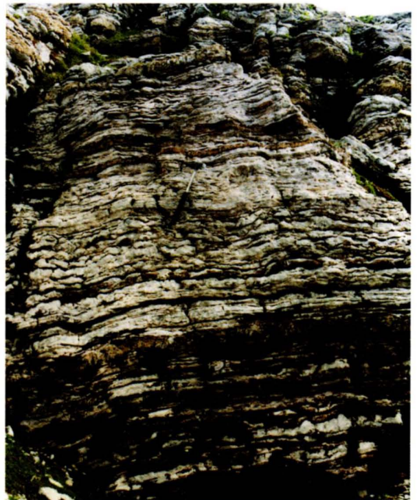
Fig. 3.68 Biancone limestone: nodular limestone with chert beds (Travnik structural unit of the Mt. Mangart saddle, section MA5).
