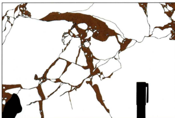
Fig. 3.80b Sketch of the neptunian dyke on the photograph 3.80a White color represents Lower Jurassic platform limestone.
