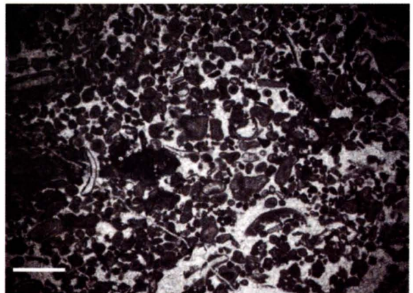
Fig. 3.8 Platform limestones: limestone with peloids, ooids, echinoderm fragments, fragments of bivalves and benthic foraminifers (section TV4). Scale bar is 1 mm long.
