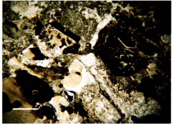
Fig. 3.59 Member 3 of the Travnik Formation: carbonate breccia with lithoclasts of Member 1 and 2 of the Travnik Formation, Sedlo Formation and fragments of stromatoporoids (section MA1). Scale bar is 1 mm long.
