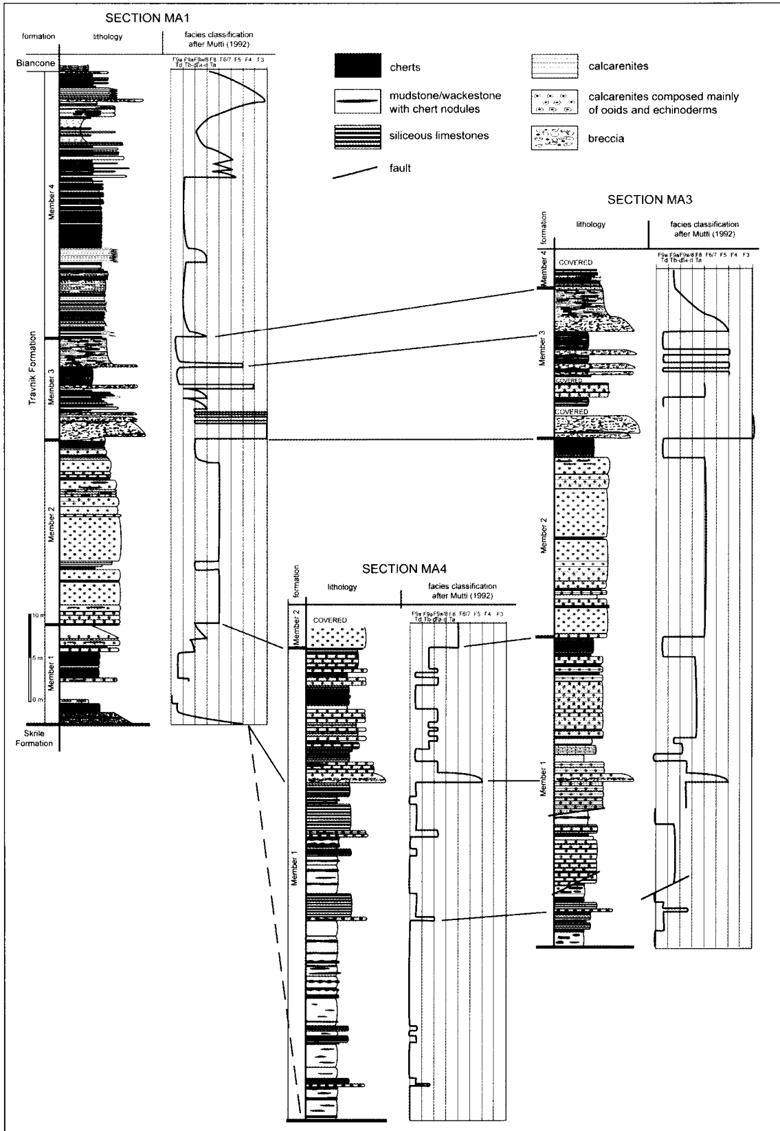
Fig. 3.49 Correlation of the Travnik Formation: MA1, MA3, and MA4 sections.
