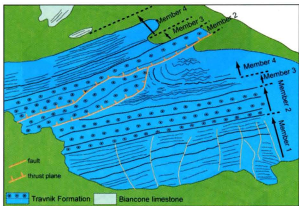
Fig. 2.10b Structural sketch of the photograph in Fig. 2.10a.
